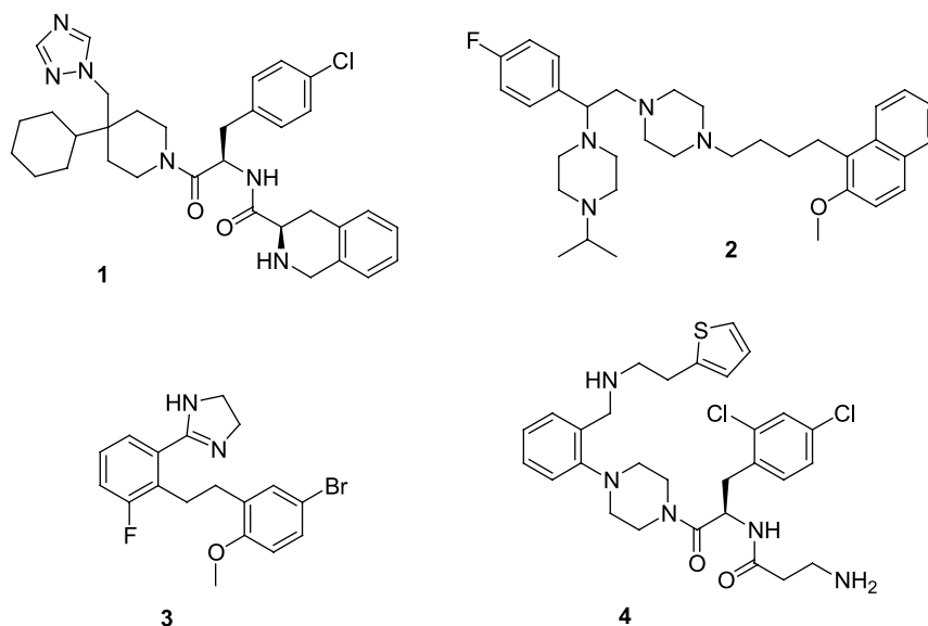
Figure 1. Some small molecule MC4R ligands.
